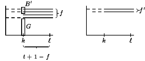
The run \rho_2 .
