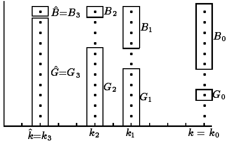
Figure 4: An example of the construction for t = 9 .
