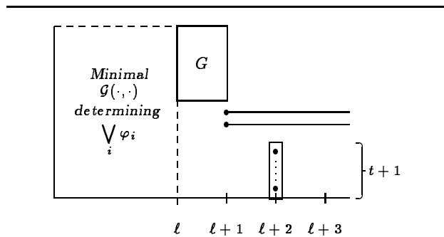
Figure 5: Embedding a graph G in a run \rho .
