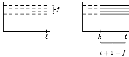
The run \rho_1 .
